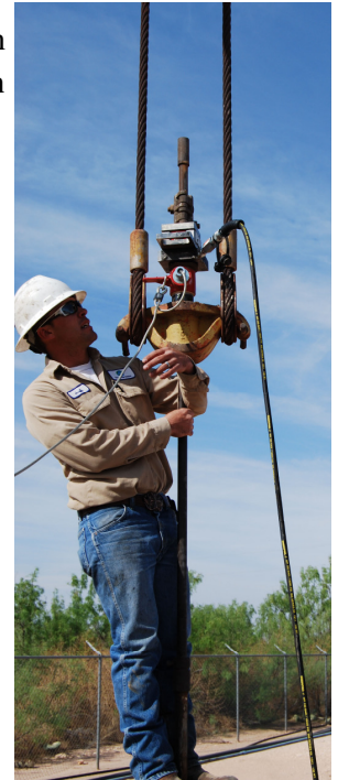
Horseshoe Load Cell in operation with String Transducer
